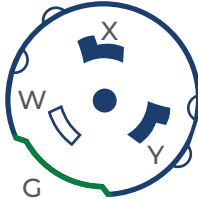
NEMA SS2-50R RECOMMENDED OPTION
